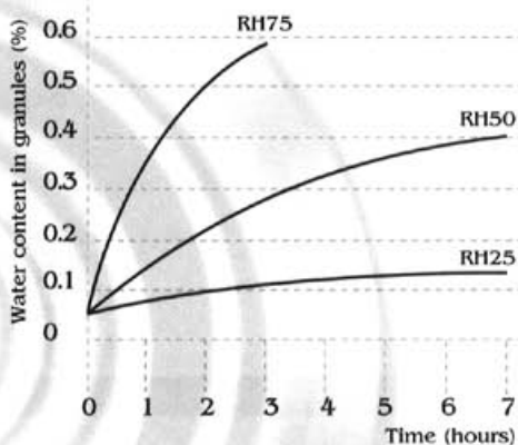
Rate of water absorption by granules at 23°C
