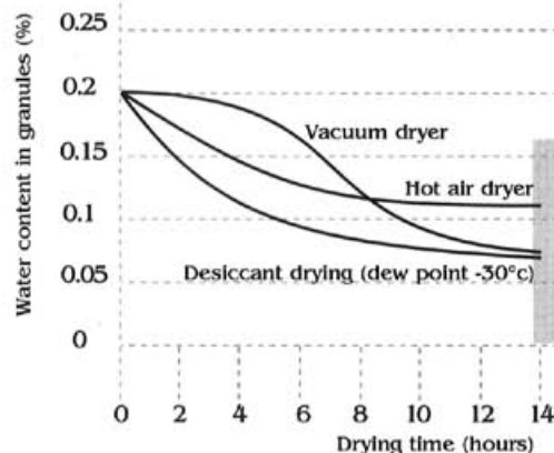
Different ways of drying
