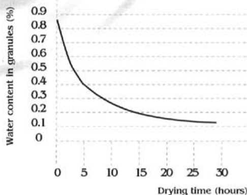
Drying very humid granules
