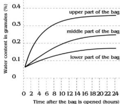
Water absorption by granules after the bag is opened
